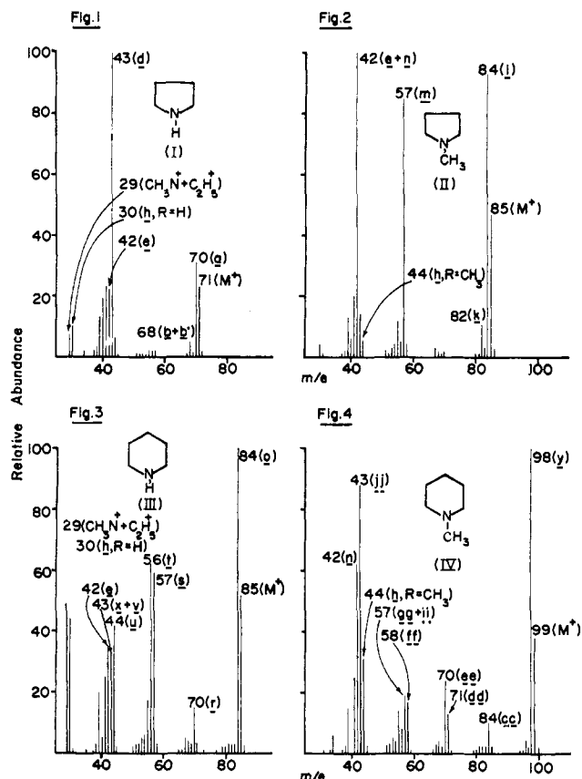
Figure 1. Mass spectrum of pyrrolidine.
